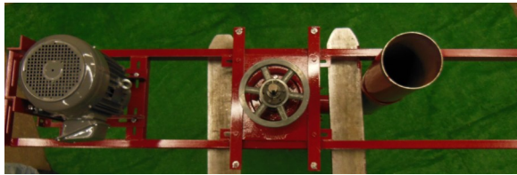
Pump with Motor and Sheaves on the mounting base ready for
