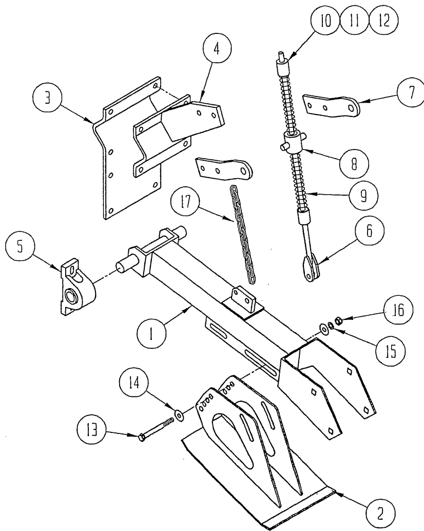
SCALPER ARM ASSEMBLY (Ground Driven & Hydraulic Driven Scalpers)
