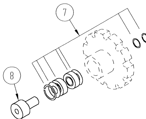
IDLER SPROCKET ASSEMBLY 10T 50MM PART #266120
