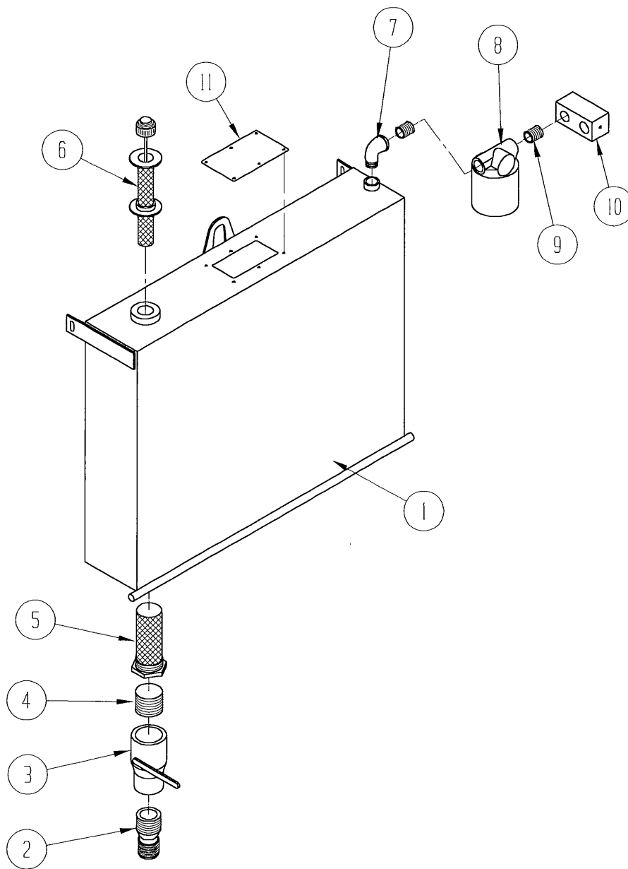
OIL RESERVOIR ASSEMBLY (SELF CONTAINED HYDRAULIC OPTION)
