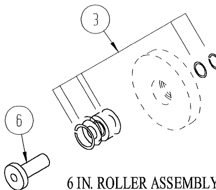
6 IN. ROLLER ASSEMBLY PART #266494
